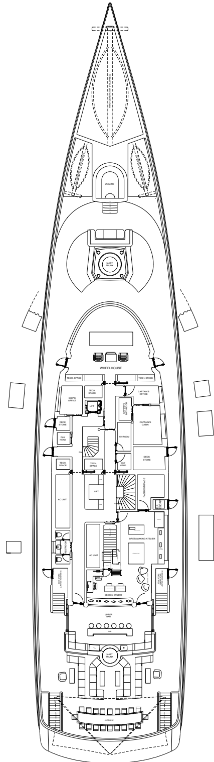
UPPER DECK
