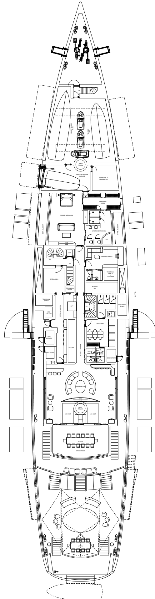
MAIN DECK
